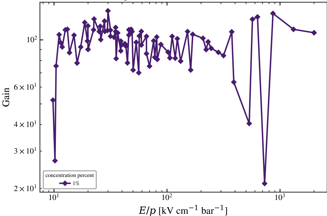
arcf4 gain vs reduced field — UNIFORM
