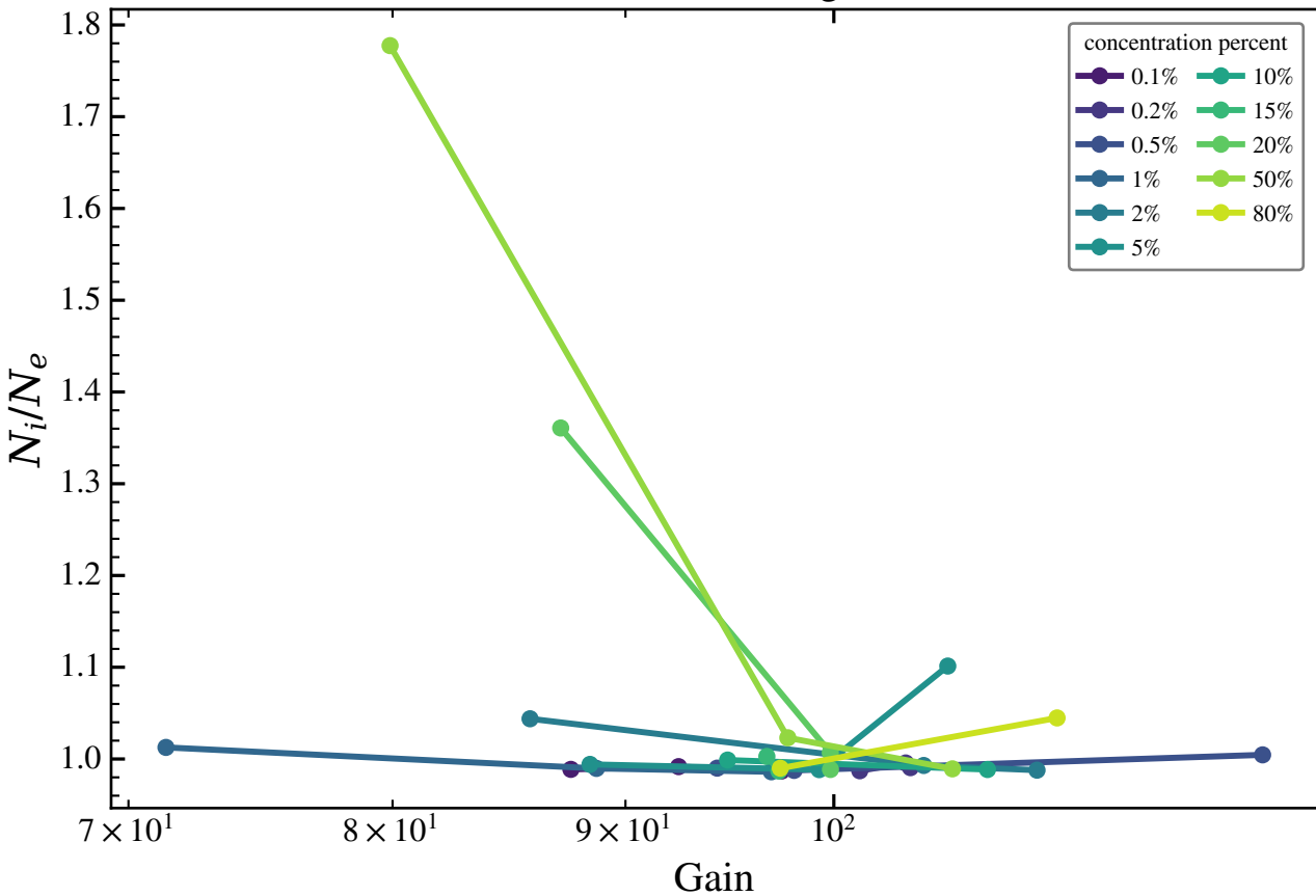
arcf4 ion electron ratio vs gain — GEM
