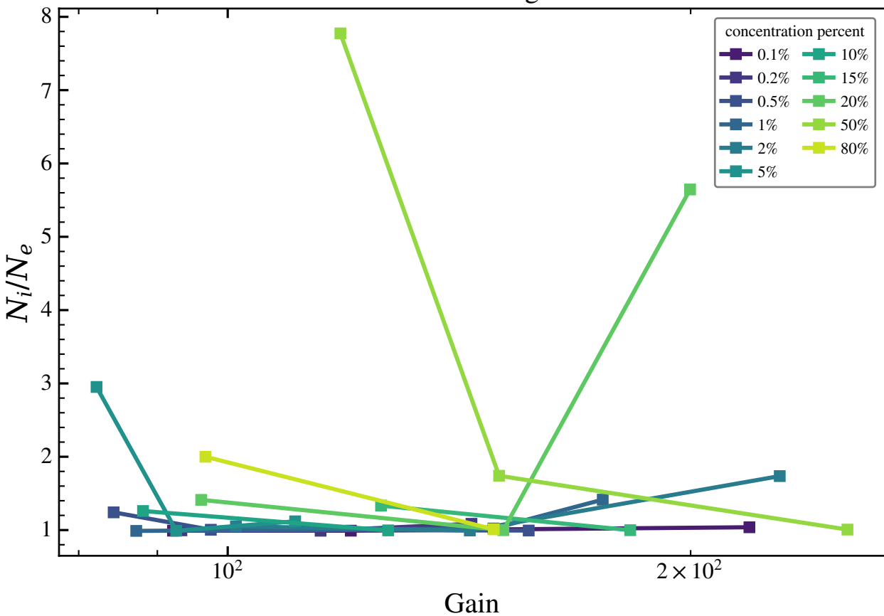
arcf4 ion electron ratio vs gain — THGEM
