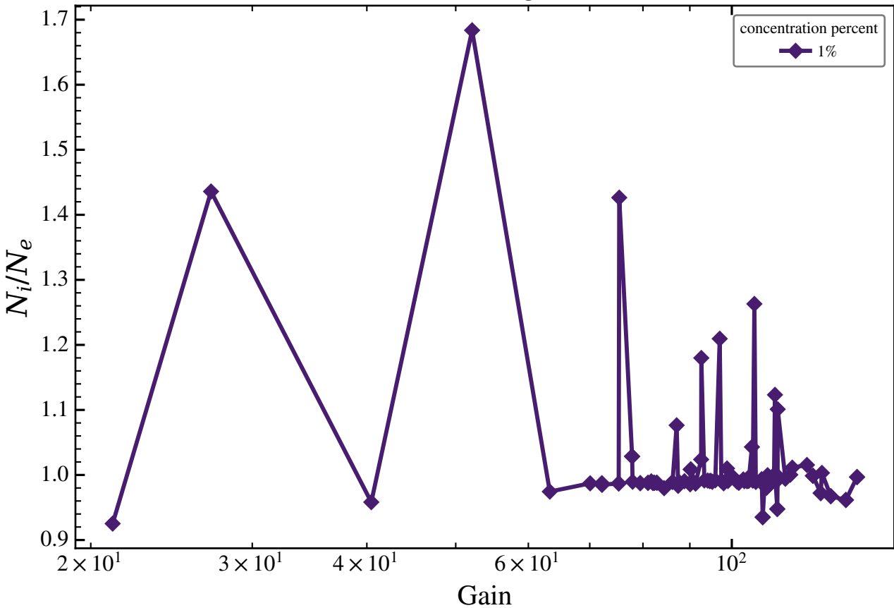
arcf4 ion electron ratio vs gain — UNIFORM
