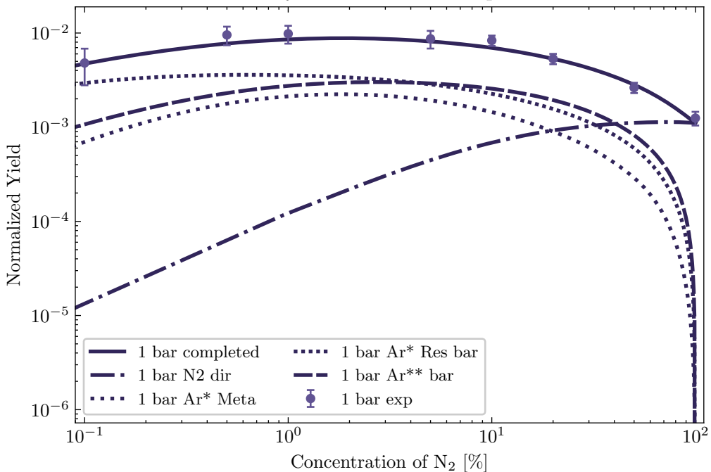
Primary ArN 2 fit 1 bar components
