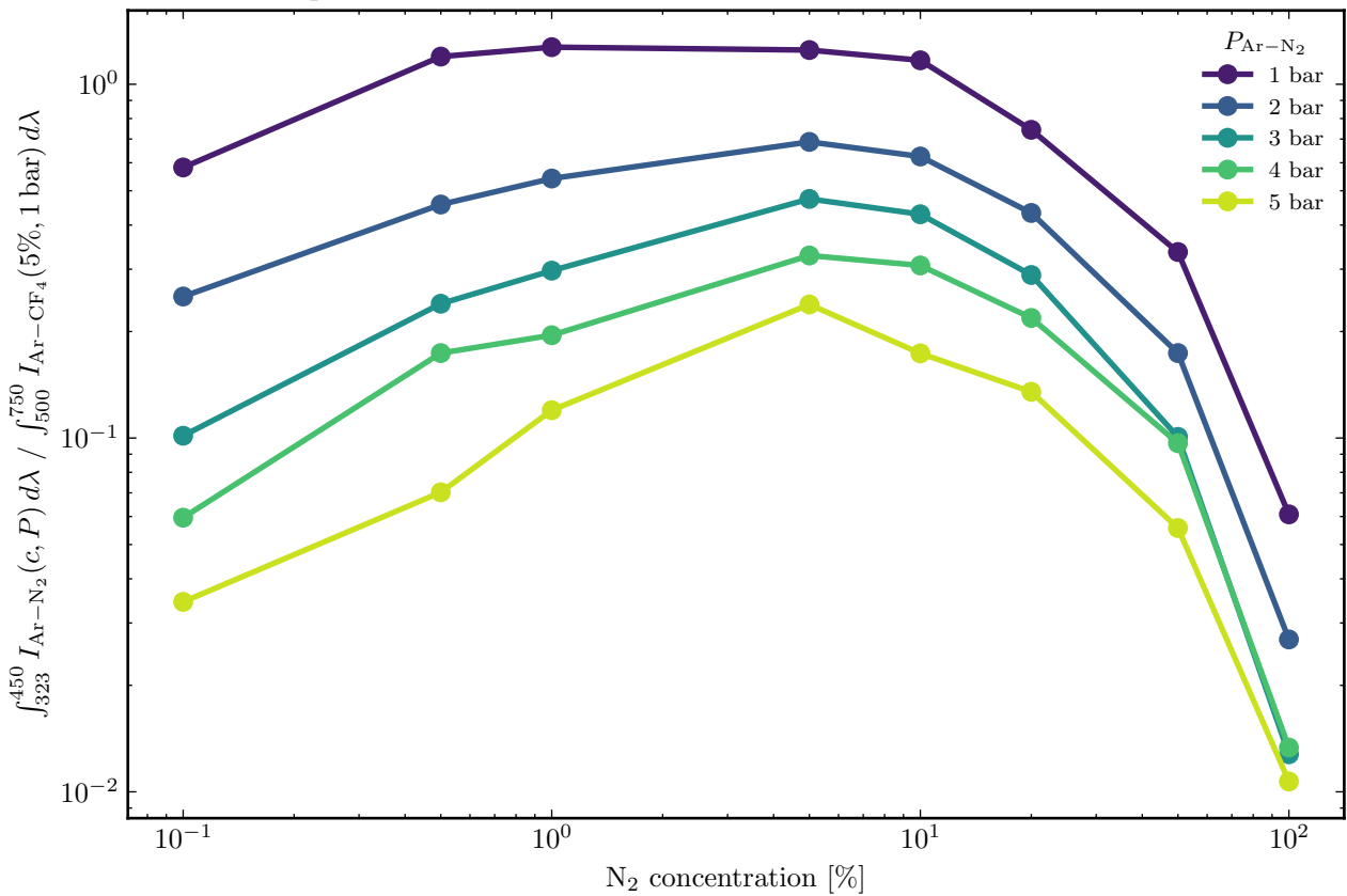
Experimental Ar-N 2 UV relative to fixed Ar-CF 4 VIS reference
