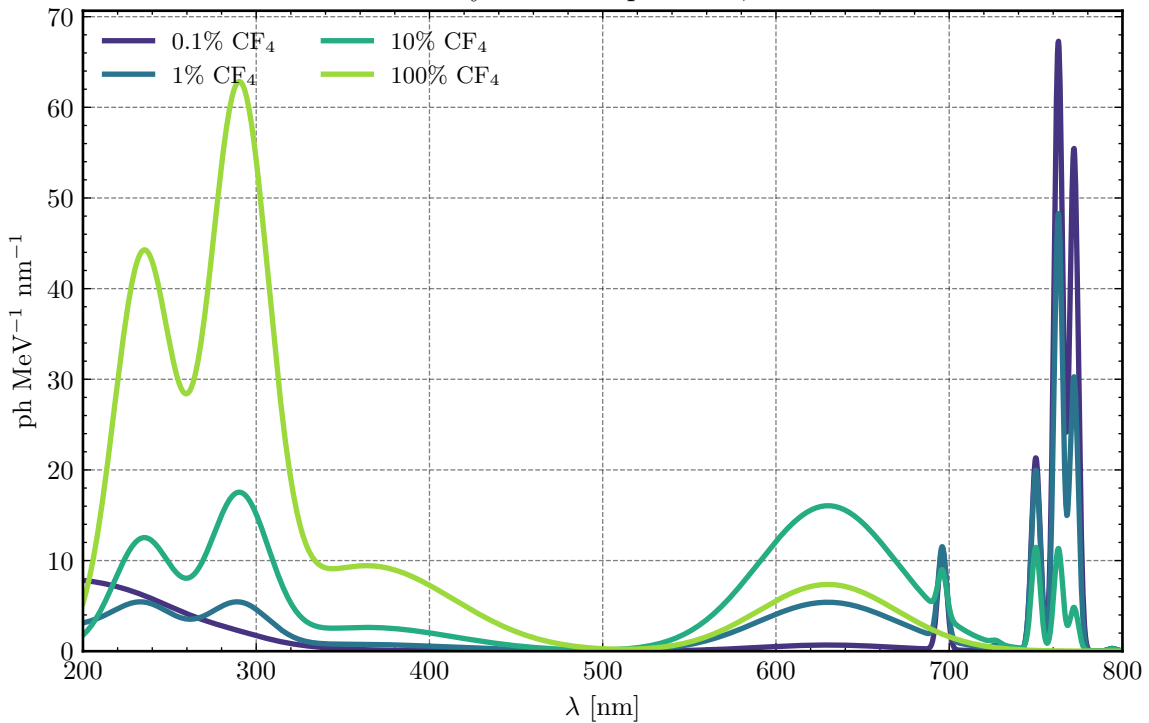
Primary Ar- \text{CF}_4 spectrum, 1 bar
