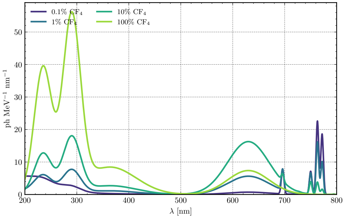
Primary Ar-CF 4 spectrum, 3 bar
