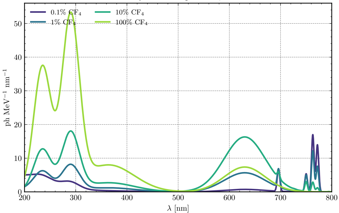
Primary Ar-CF 4 spectrum, 4 bar
