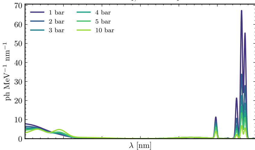
Ar-CF 4 , 10% CF 4
