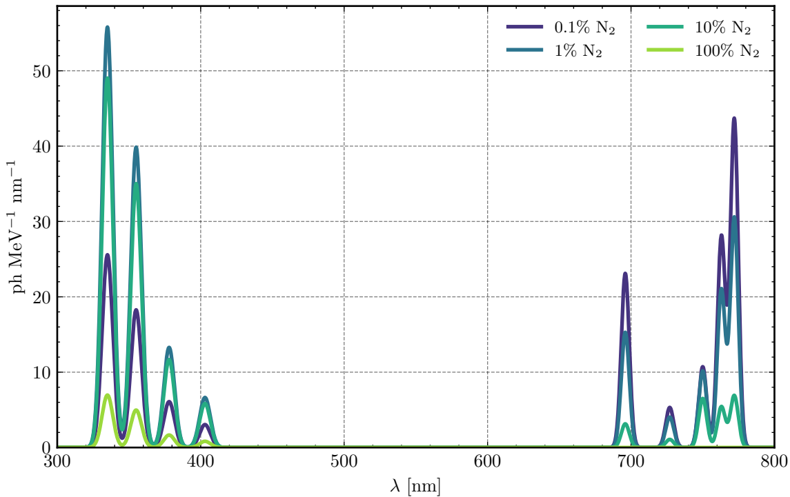
Primary Ar-N 2 spectrum, 2 bar
