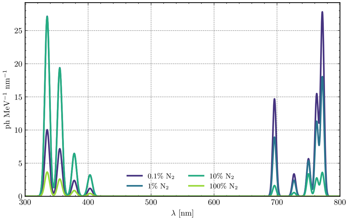
Primary Ar-N 2 spectrum, 4 bar
