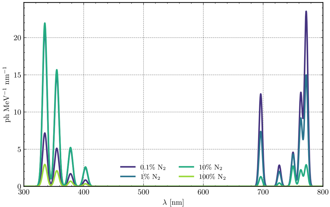
Primary Ar-N 2 spectrum, 5 bar
