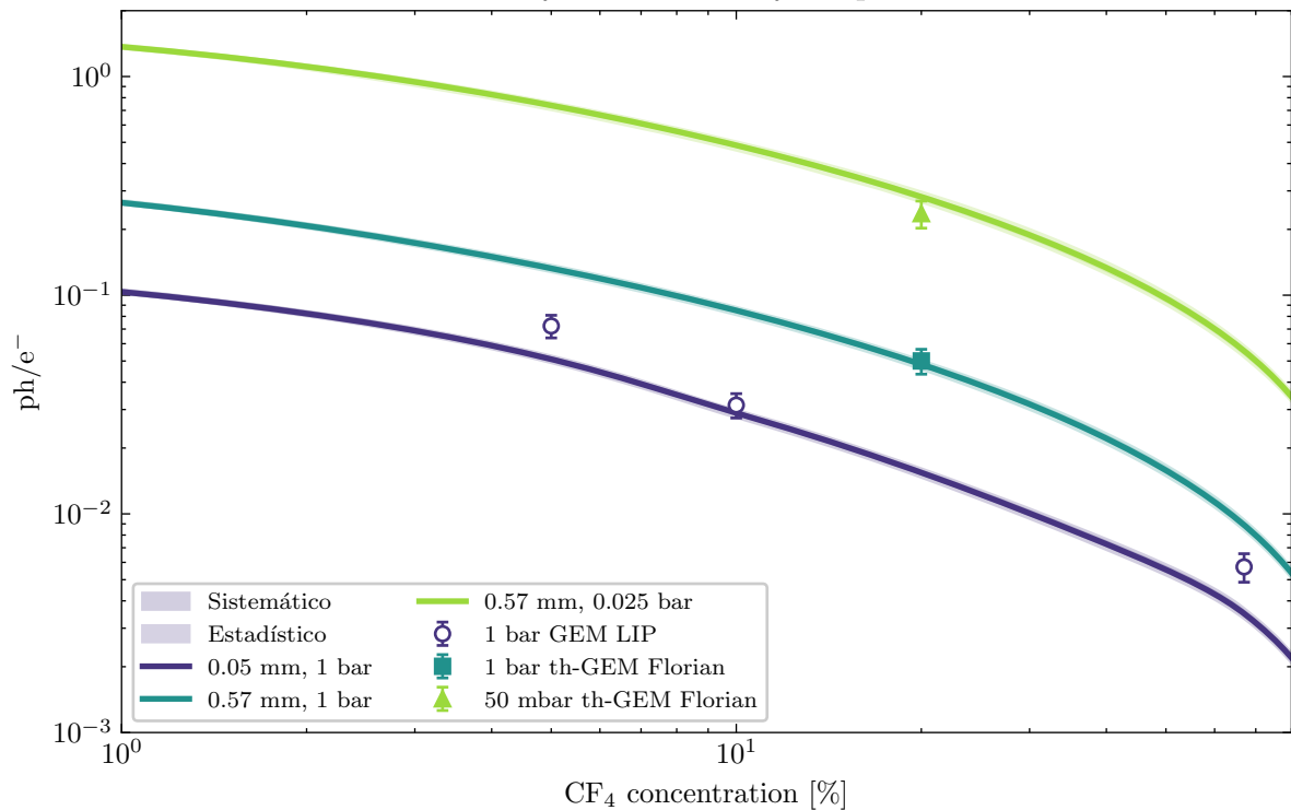
Secondary Ar- \text{CF}_4 NIR yield prediction
