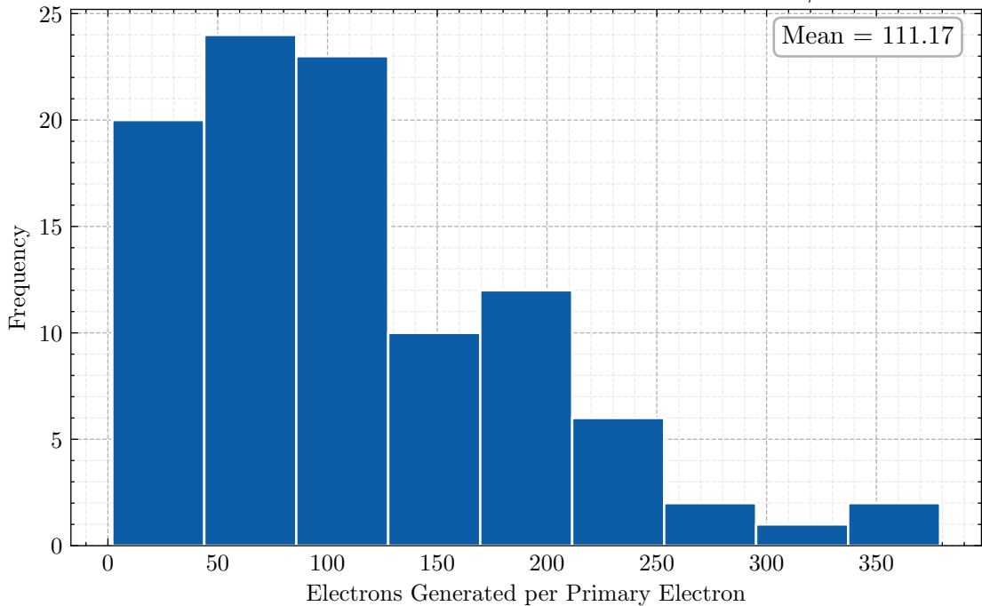
Electron Gain ar 99.0% - cf4 1.0% 1.0 bar 31.6 kV/cm
