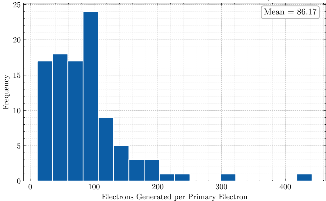
Electron Gain ar 99.0% - cf4 1.0% 1.0 bar 65.8 kV/cm
