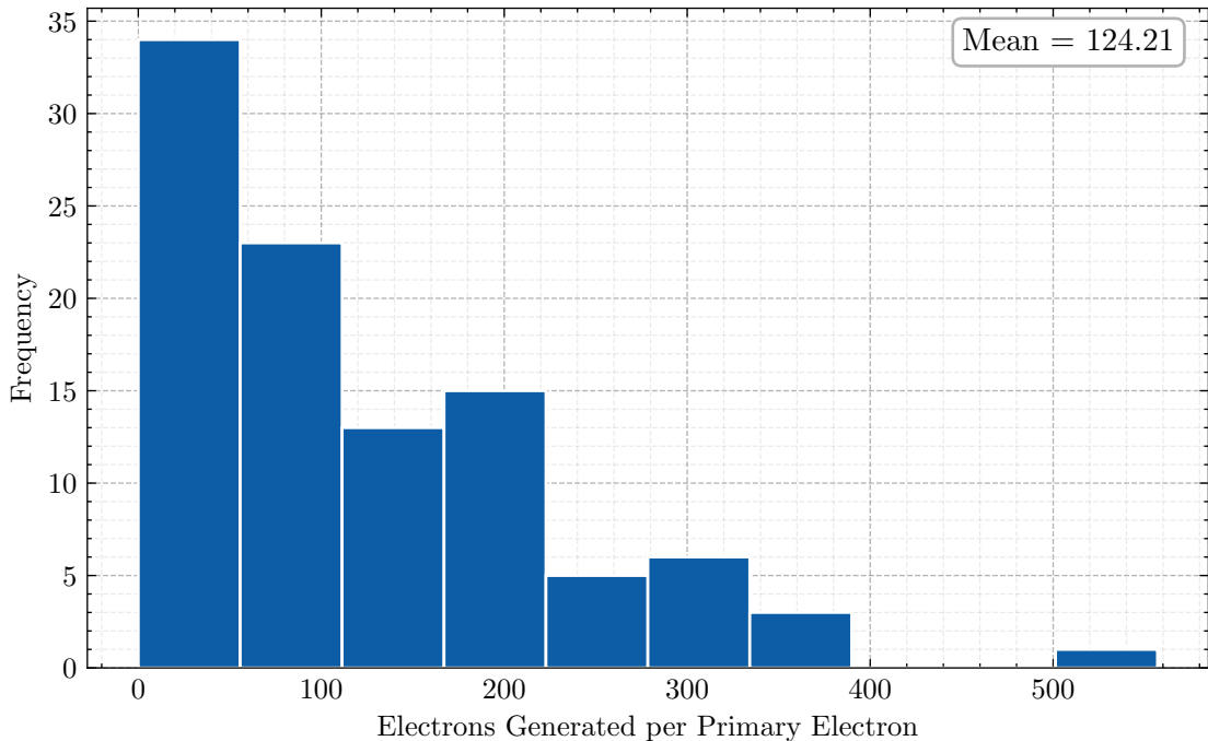
Electron Gain ar 99.5% - cf4 0.5% 10.0 bar 184.5 kV/cm
