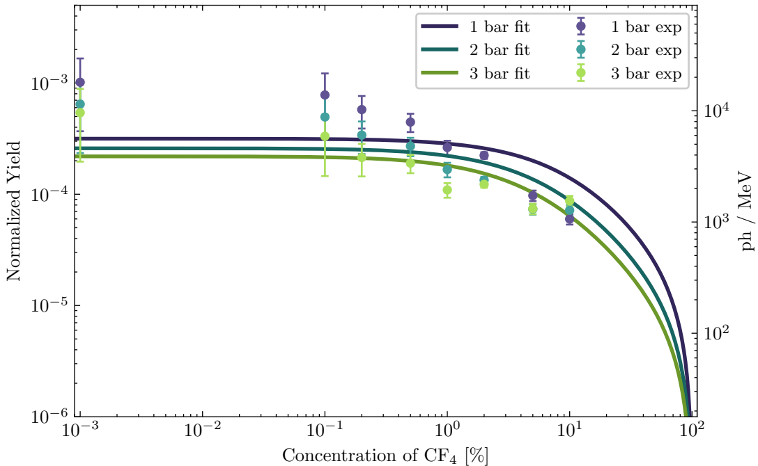
Primary ArCF 4 IR (696 nm) Yield fit
