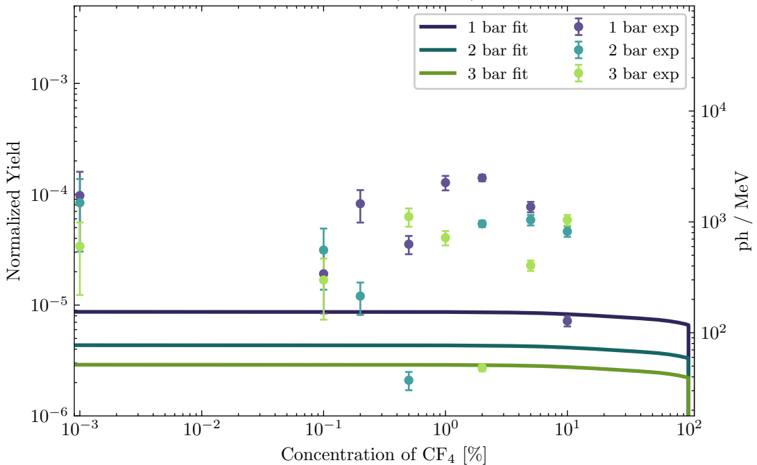
Primary ArCF 4 IR (794 nm) Yield fit
