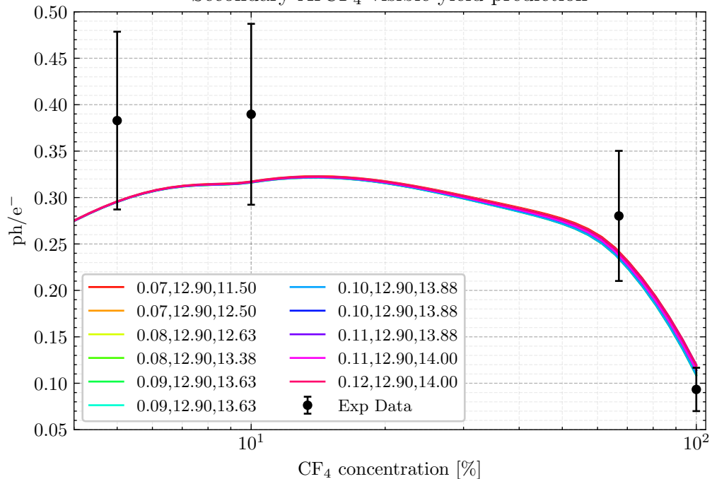
Secondary ArCF 4 visible yield prediction
