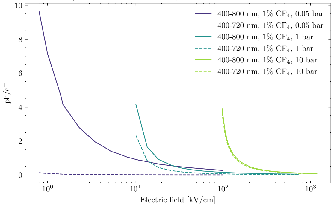
Secondary Yield Prediction for Ar/CF 4 mixture, 1% CF 4 & 100 Gain
