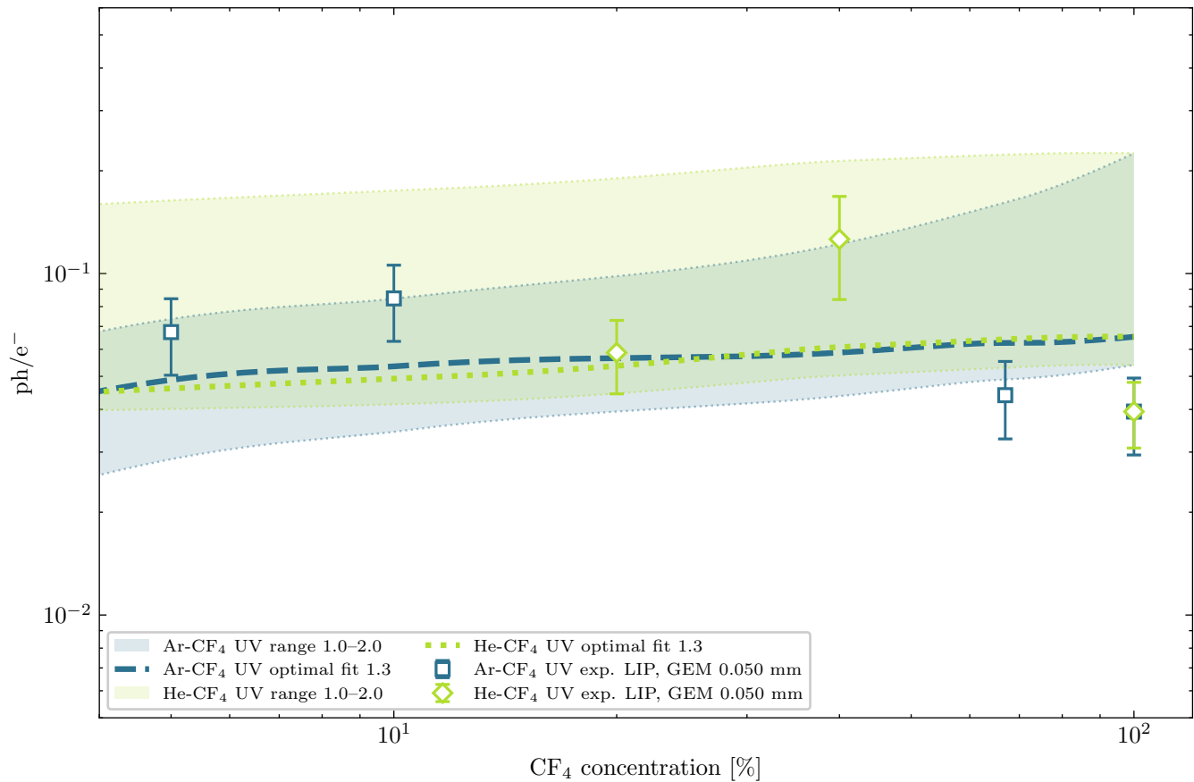
LIP GEM 0.050 mm: Ar-CF 4 and He-CF 4 UV
