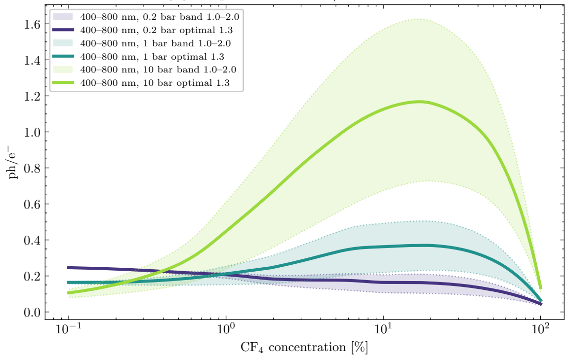
Secondary yield prediction for Ar/CF 4 GEM, 400–800 nm
