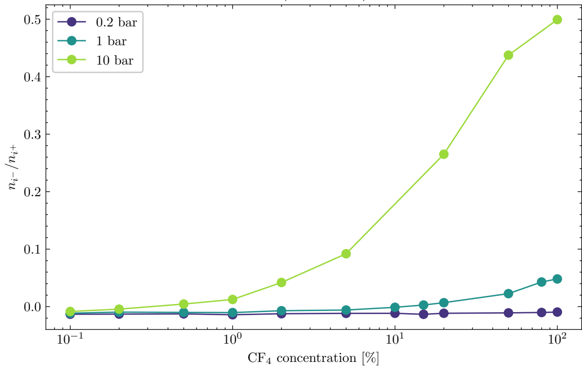
Estimated n_{i-}/n_{i+} for Ar/CF 4 GEM
