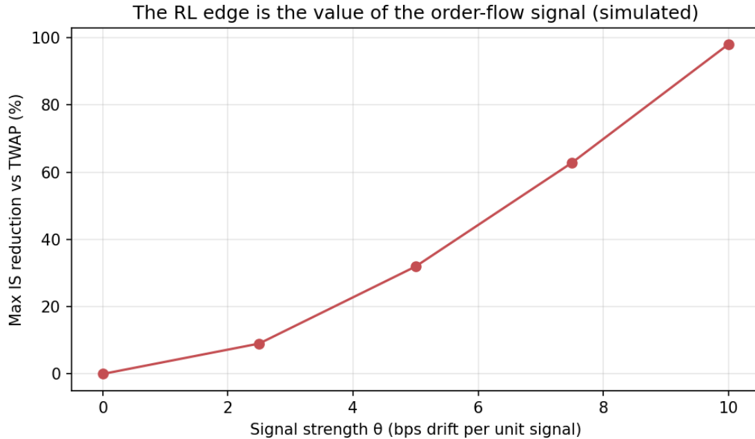
Figure 4.6, The RL edge scales with the order-flow signal strength (simulated).
