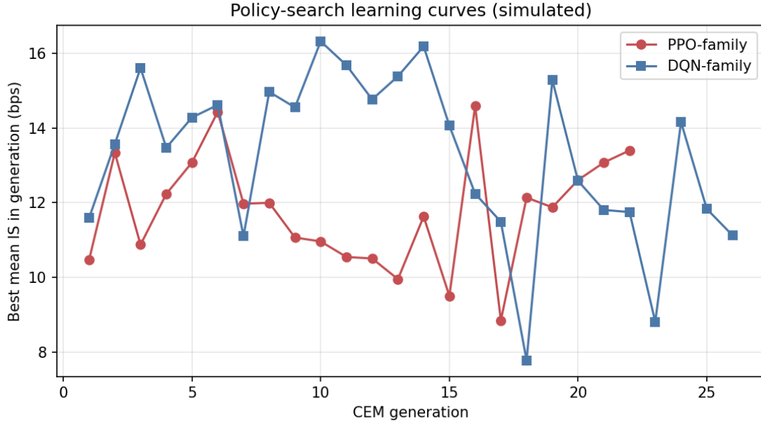
Figure 4.7, Policy-search learning curves: best mean IS per CEM generation (simulated).
