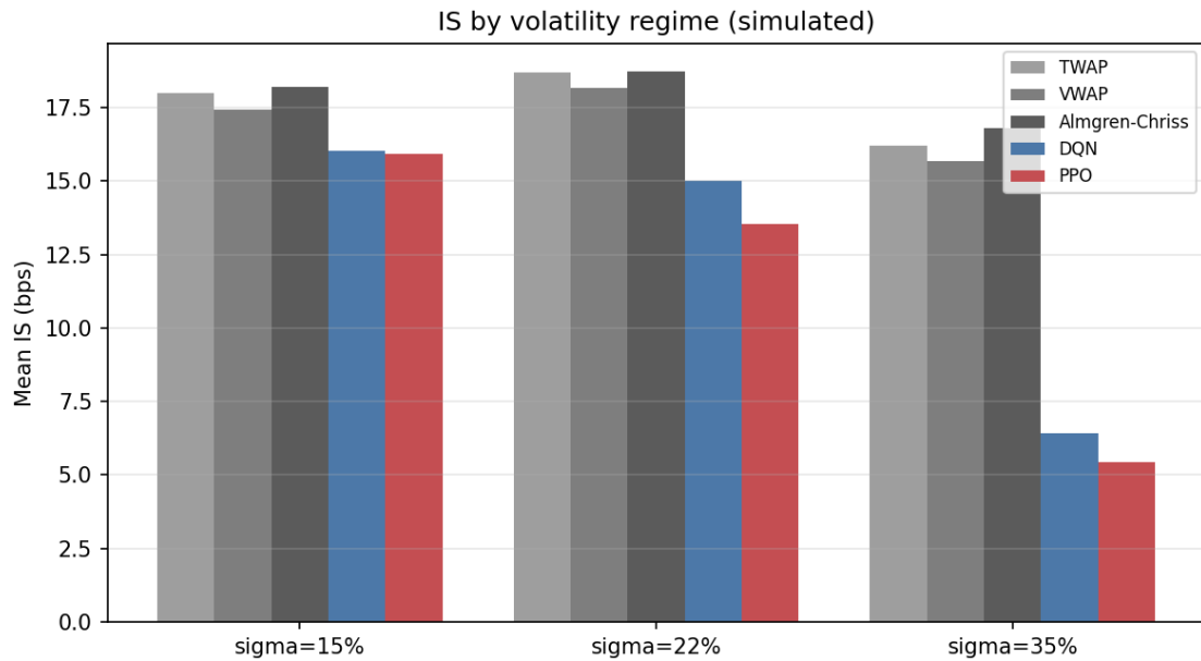
Figure 4.3, Mean Implementation Shortfall by strategy and volatility regime (simulated).
