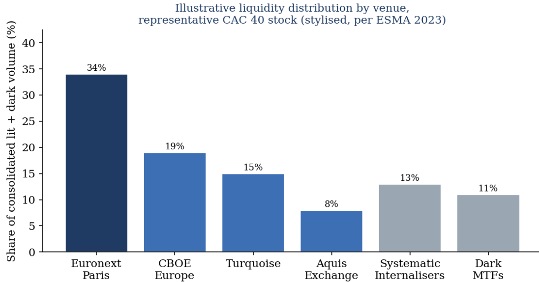
Figure 1.3, Illustrative liquidity distribution by venue for a representative CAC 40 stock (stylised, consistent with ESMA 2023).
