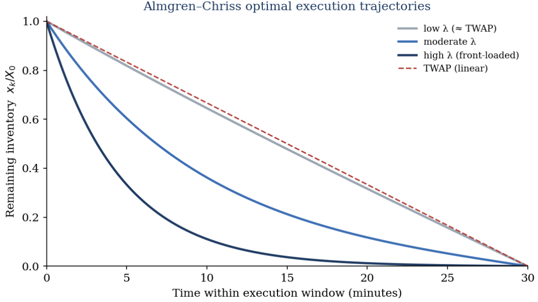
Figure 1.2, Optimal execution trajectories under Almgren-Chriss (2001) for different values of risk aversion \lambda ; larger \lambda leads to faster front-loading.
