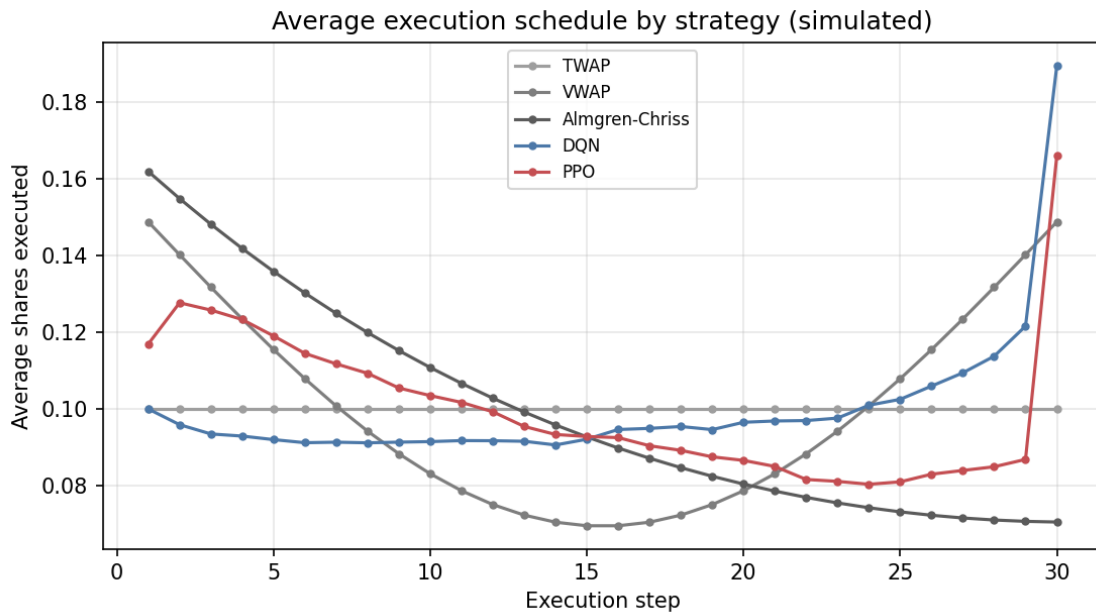
Figure 4.2, Realised average execution schedule by strategy in the out-of-sample evaluation (simulated).
