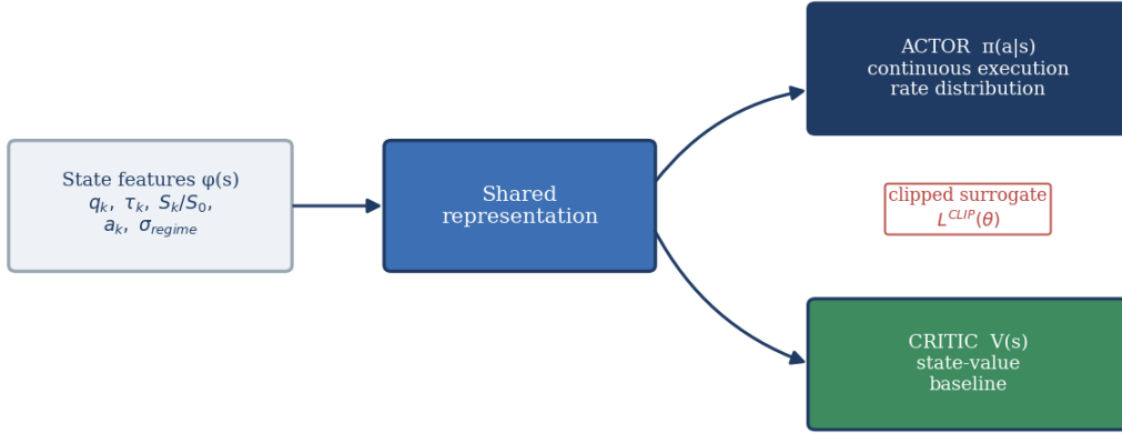
Figure 1.4, Shared actor-critic architecture of the PPO algorithm, adapted from Schulman et al. (2017).
