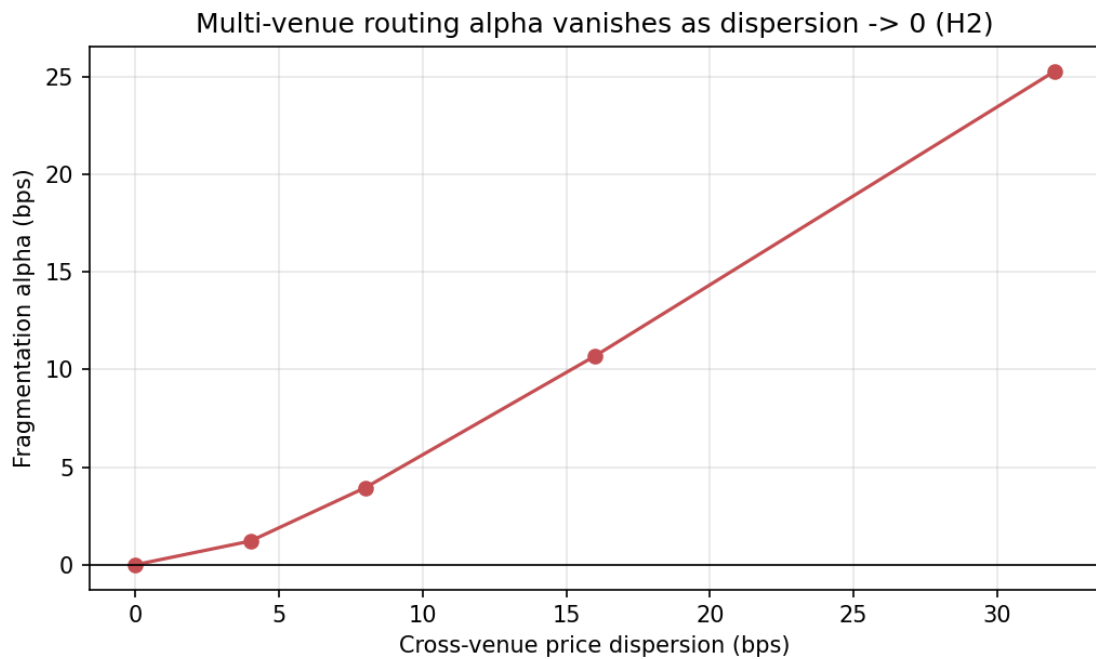
Figure 4.5, Fragmentation alpha vanishes as cross-venue dispersion approaches zero (H2).
