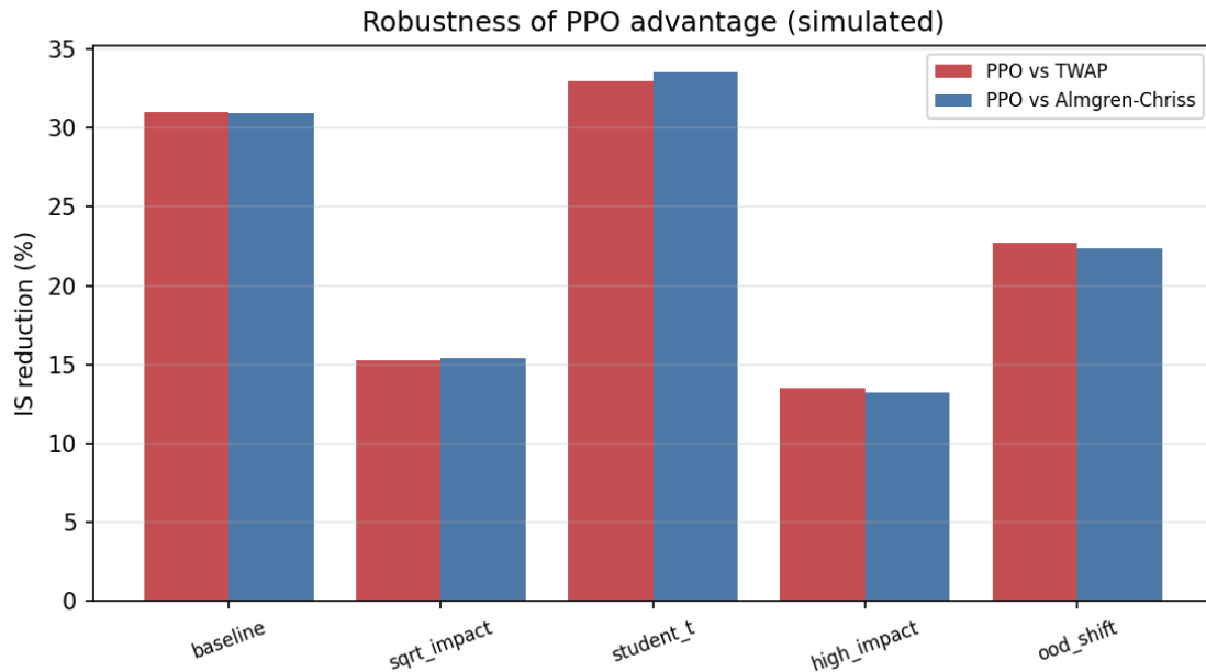
Figure 4.8, Robustness of the PPO advantage across model assumptions (simulated).
