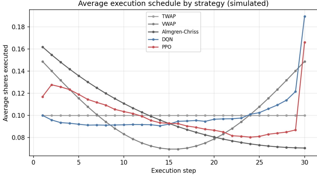
Figure 3.2, Average execution schedule by strategy (simulated).
