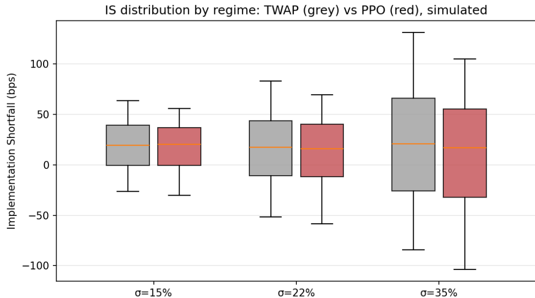
Figure 4.4, IS distribution by volatility regime: TWAP vs PPO (simulated).
