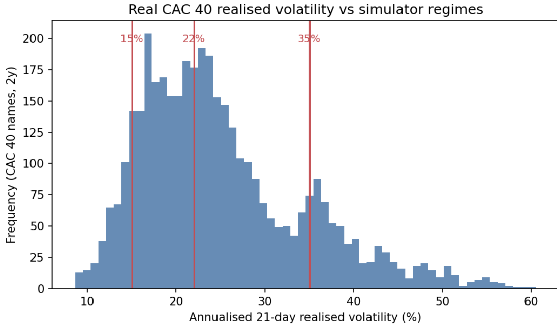
Figure 3.3, Real CAC 40 21-day realised volatility (eight constituents, two years) with the simulator's three volatility regimes (15%, 22%, 35%) marked.
