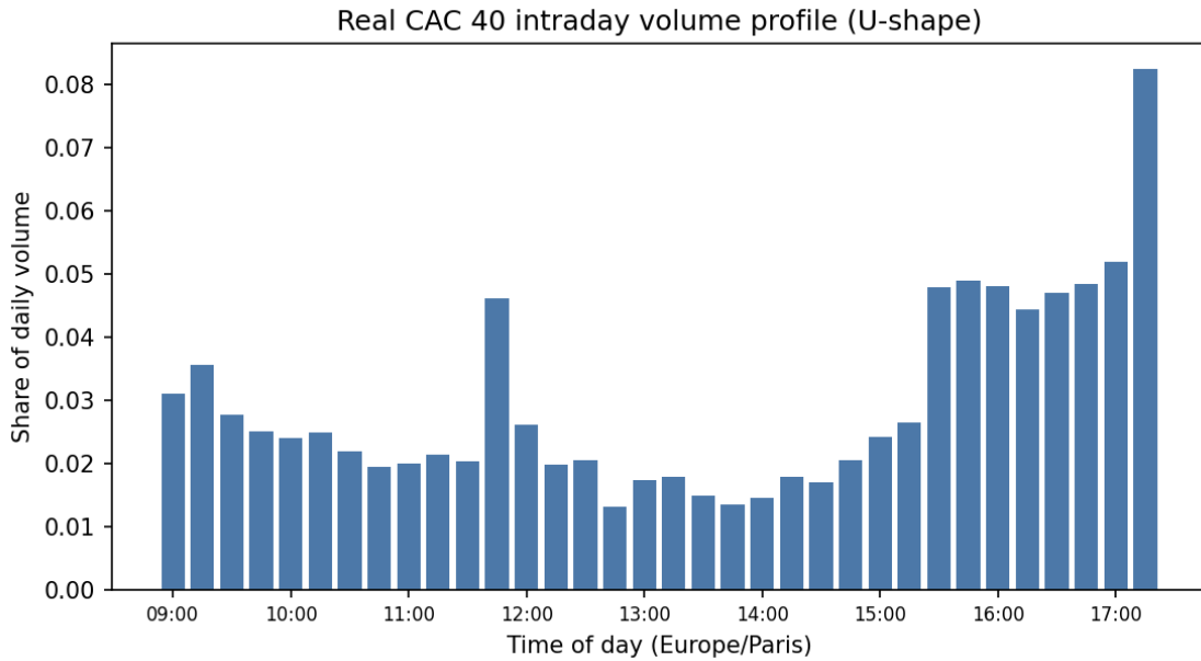
Figure 3.4, Real CAC 40 intraday volume profile, confirming the U-shape assumed by VWAP and the seasonality term.
