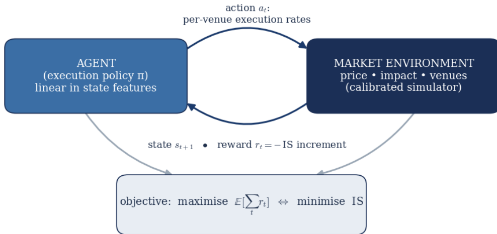
Figure 2.1, MDP architecture for the multi-venue optimal execution problem, adapted from Sutton & Barto (2018) and
