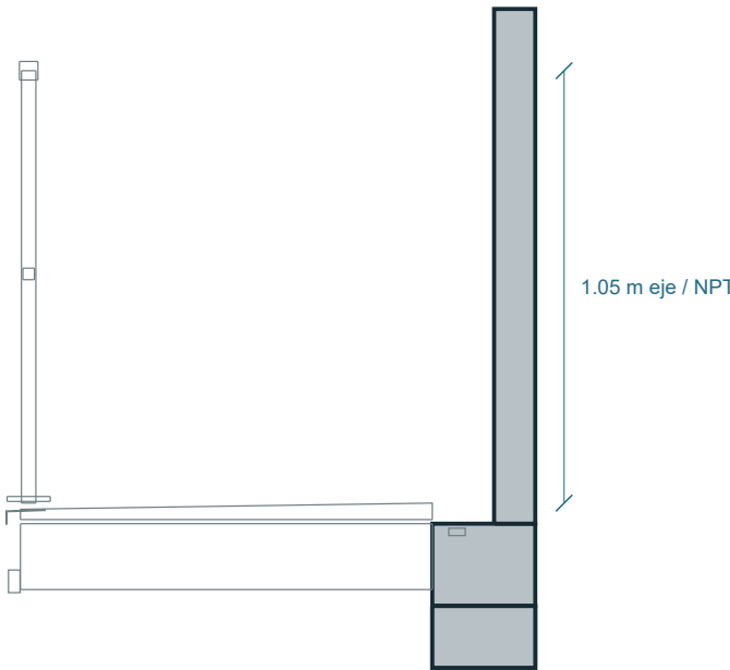
D04 Balcon / baranda / Z=9,00 | 1:20
