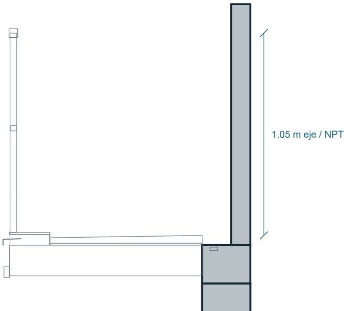
04/A14 Balcon / baranda / Z=9,00 | 1:20
