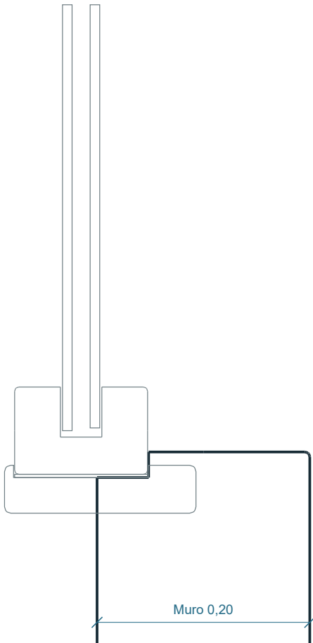
06/A13b DVH / antepecho / Z=3,00 | 1:5
