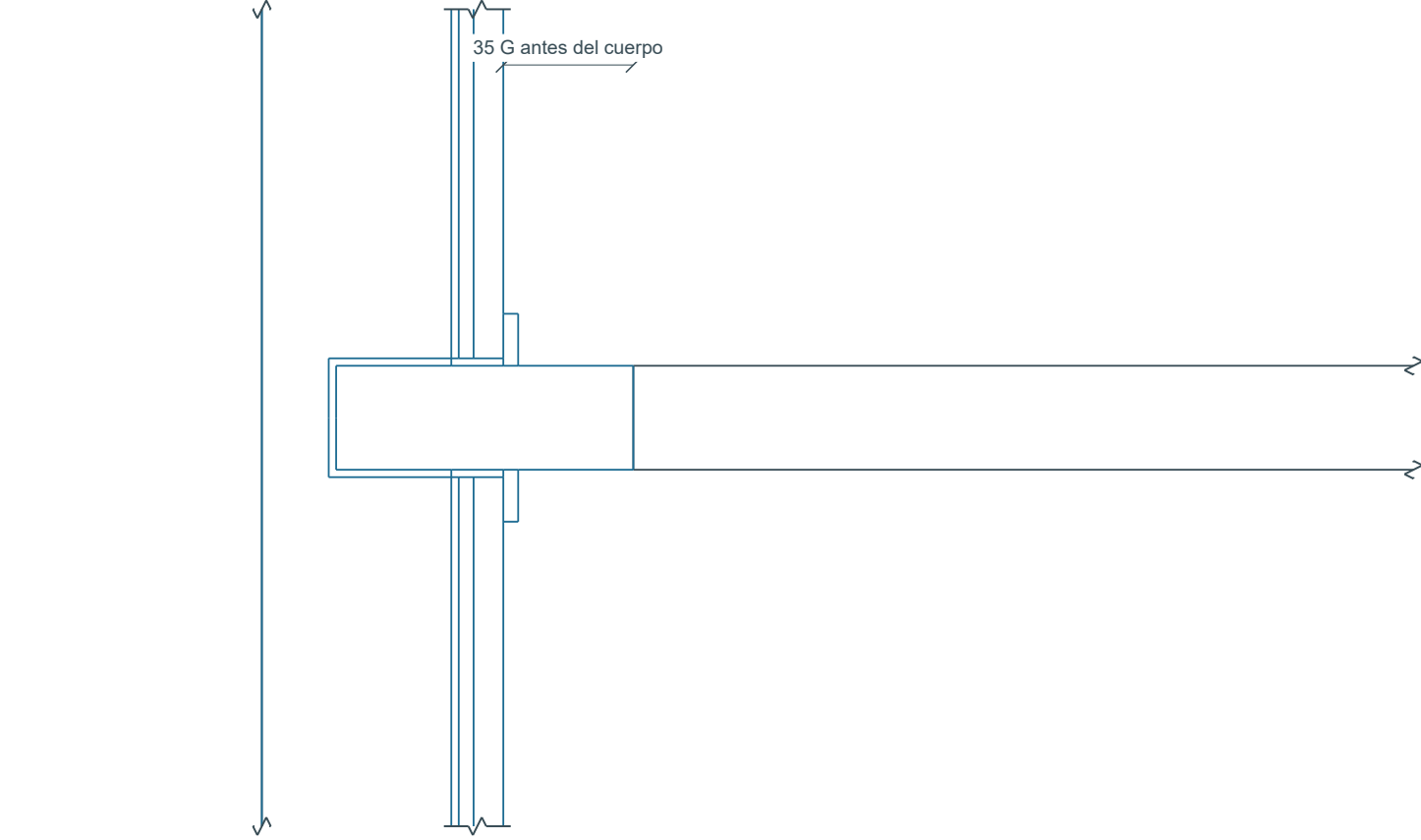
26 Griferia PA / X21,10 | 1:2
