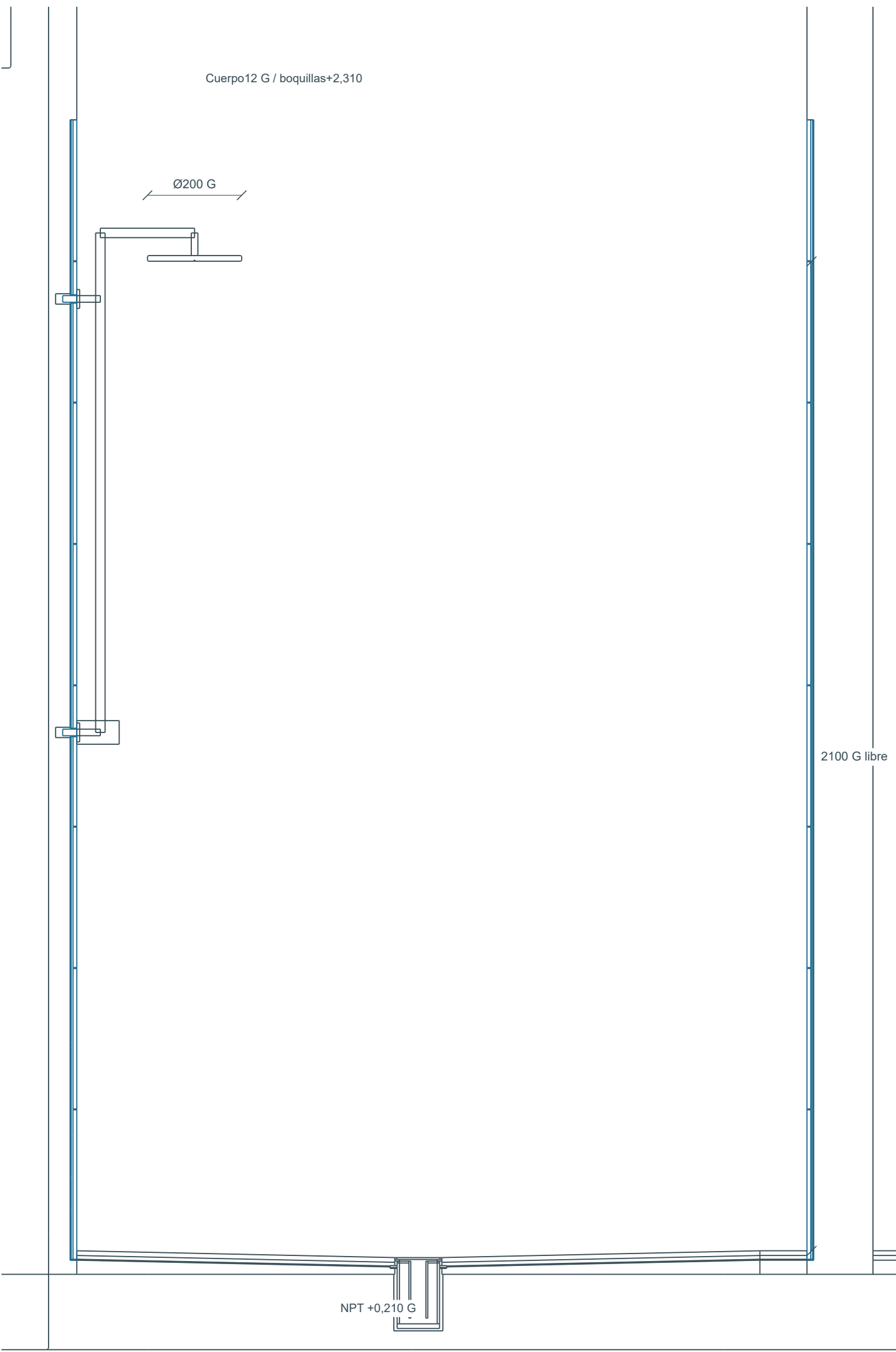
25 Ducha PB / X21,35 | 1:10
