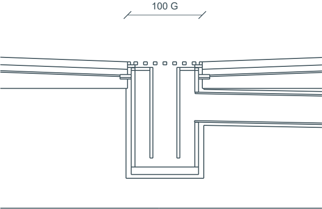
28 Sumidero PB / Z0,985 | 1:5
