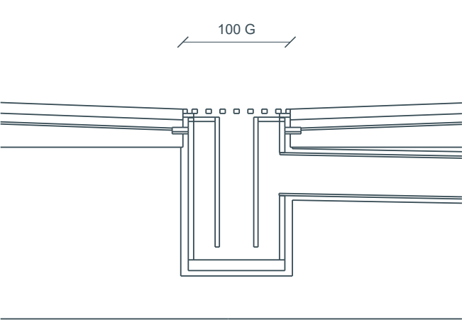
28 Sumidero PB / Z0,985 | 1:5
