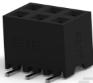
TE Part #2314844-6 6P,2MM,B-B,REC,DRVT,SMD,0.1AU, TB,W/CP
