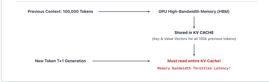
DIAGRAM 1.4: THE AUTOREGRESSIVE GENERATION PIPELINE & KV CACHE
