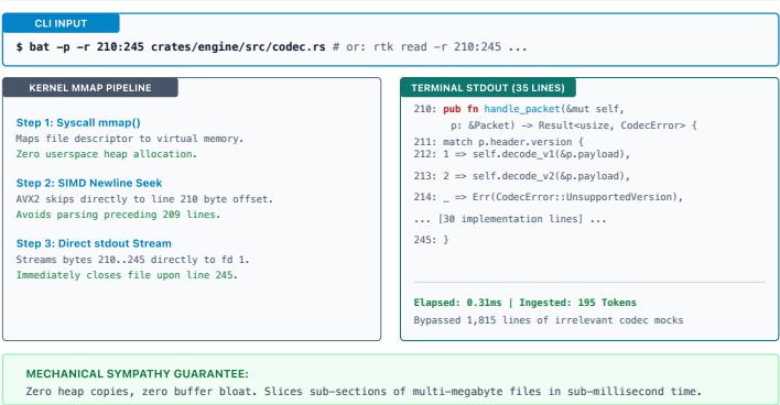
DIAGRAM 6.4: THE BAT SLICING & MMAP EXTRACTION PIPELINE (CLI INPUT & OUTPUT)
