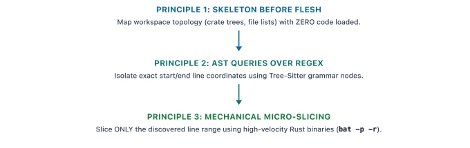
DIAGRAM 3.5: THE THREE CORE PRINCIPLES OF CONTEXT SLICING
