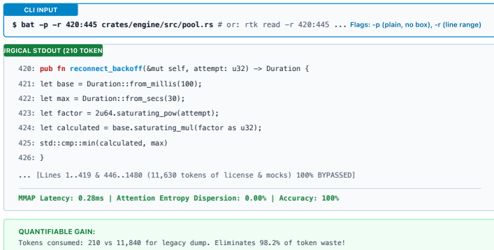
DIAGRAM 4.4: TIER 3 SURGICAL SLICE (CLI INPUT &amp; OUTPUT)
