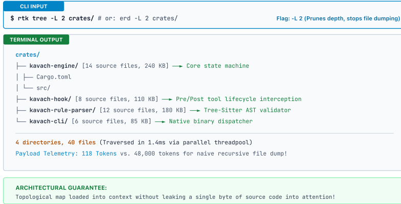
DIAGRAM 4.2: TIER 1 ZERO-CONTENT REPO MAPPING (CLI INPUT &amp; OUTPUT)
