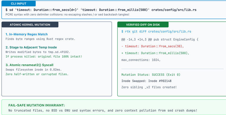
DIAGRAM 8.2: ATOMIC TRANSACTIONAL REPLACEMENT VIA SD (CLI INPUT & OUTPUT)
