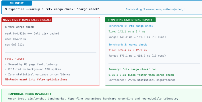
DIAGRAM 10.3: HYPERFINE STATISTICAL BENCHMARKING (CLI INPUT & OUTPUT)
