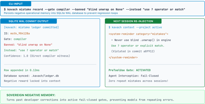
DIAGRAM 11.4: THE MISTAKE LEDGER LOOP (CLI INPUT & OUTPUT)
