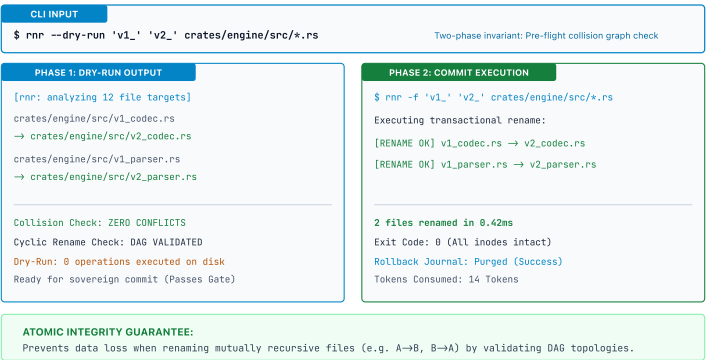
DIAGRAM 8.3: RNR TWO-PHASE TRANSACTIONAL RENAMING (CLI INPUT & OUTPUT)
