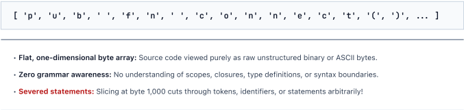
DIAGRAM 3.1: THE NAIVE VIEW OF CODE (FLAT CHARACTER STREAM)
