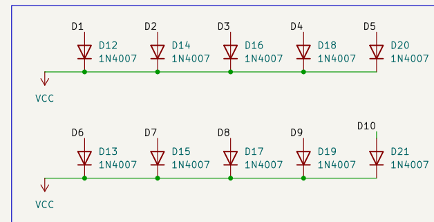
Flyback Diodes
