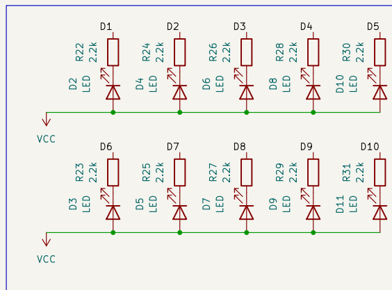
Output Indicators LED
