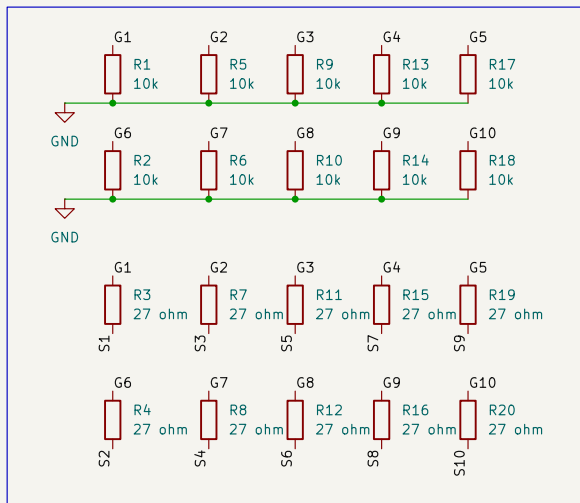
Gate Resistors and Pull Down Resistors
