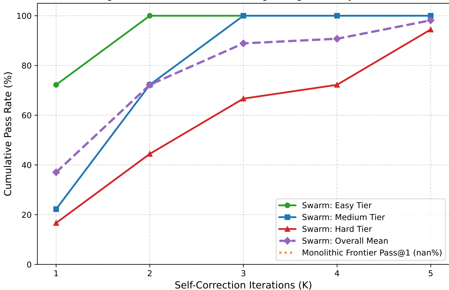
Figure 1: Iteration Count vs. Bug-Fixing Accuracy Curve
