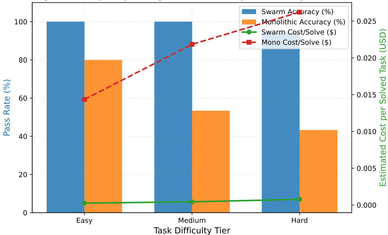
Figure 2: Complexity Ceiling Break-Even Analysis (Accuracy vs. Cost)
