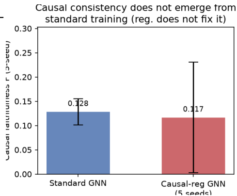
Fig. 1. Five-seed causal faithfulness (fraction of toxicophore removals that drop the prediction by \geq 0.1 ). BBBP: standard GNN and causal-regularized GNN are statistically indistinguishable (0.128 \pm 0.027 vs 0.117 \pm 0.114, Welch p = 0.83 ); the regularizer adds instability, not faithfulness. On BACE the regularizer is significantly worse than baseline (0.477 \pm 0.061 vs 0.195 \pm 0.195, Welch p = 0.029 ). Error bars = sample std. See Table II for the full cross-dataset comparison.
