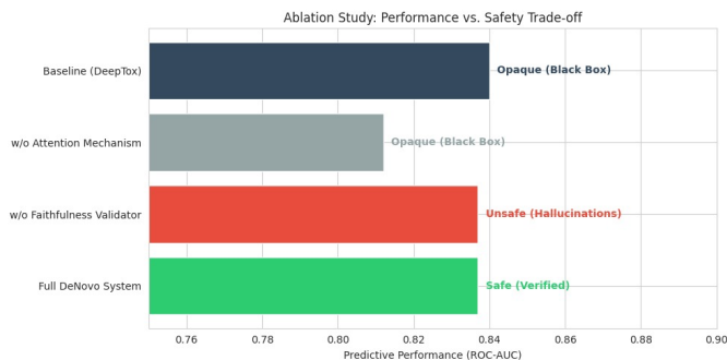
Fig. 5. Ablation Study results. The full DeNovo system (green) balances accuracy with verified safety.
