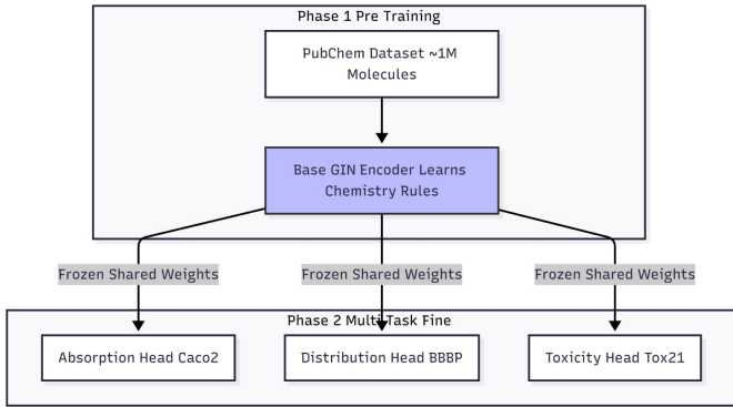
Fig. 3. Transfer Learning Strategy. The encoder is pre-trained on 1M molecules using context prediction, then fine-tuned with task-specific heads for ADMET prediction.
