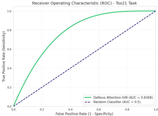
Fig. 4. ROC curve for Tox21 prediction (validation AUC = 0.837; test AUC = 0.802), indicating strong class separability.
