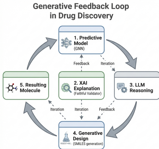
Fig. 7. Proposed Generative Feedback Loop. The Faithfulness Validator provides grounded feedback to a generative agent, guiding the optimization toward molecules with high efficacy and low toxicity.
