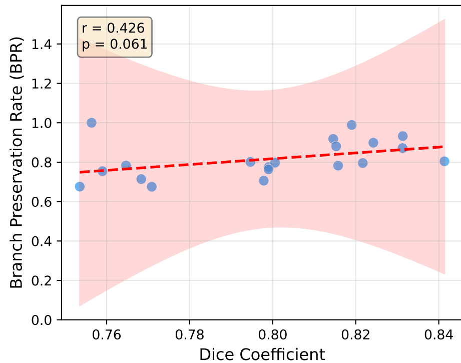
U-Net (DRIVE)
