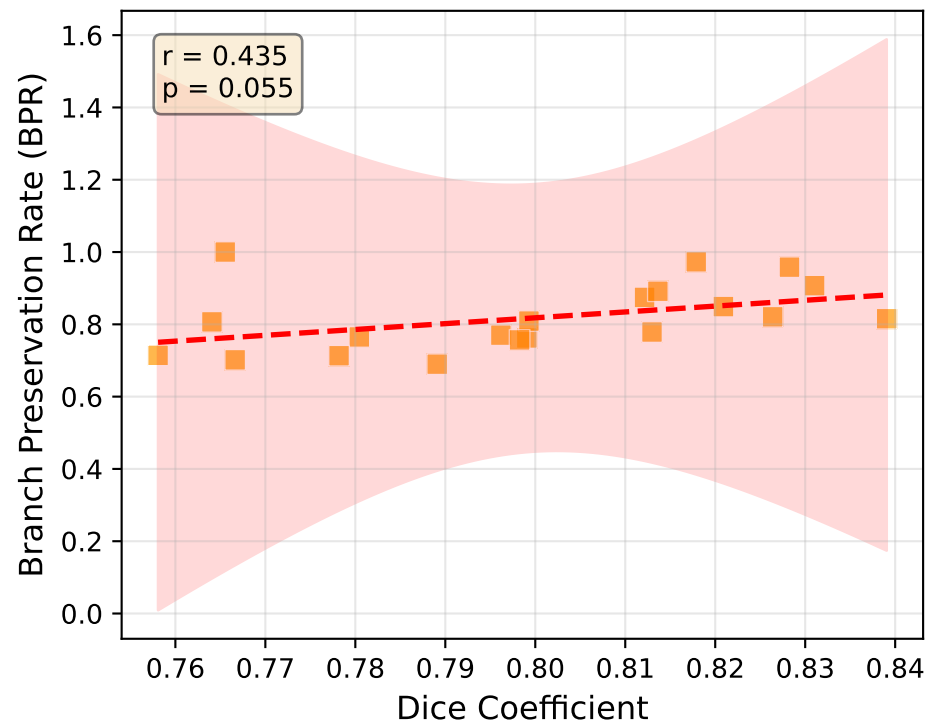
UNet++ (DRIVE)
