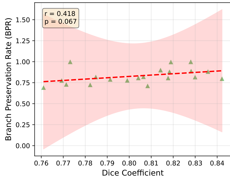
Retina-UNet (DRIVE)
