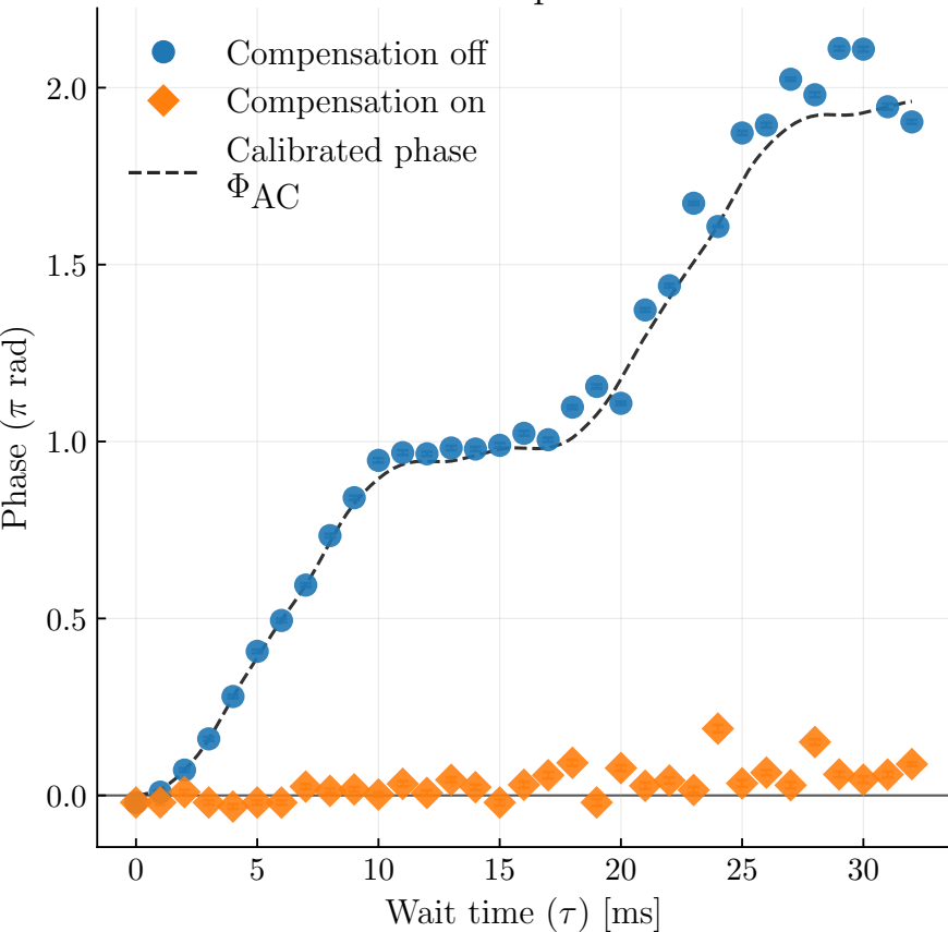
Phase compensation
