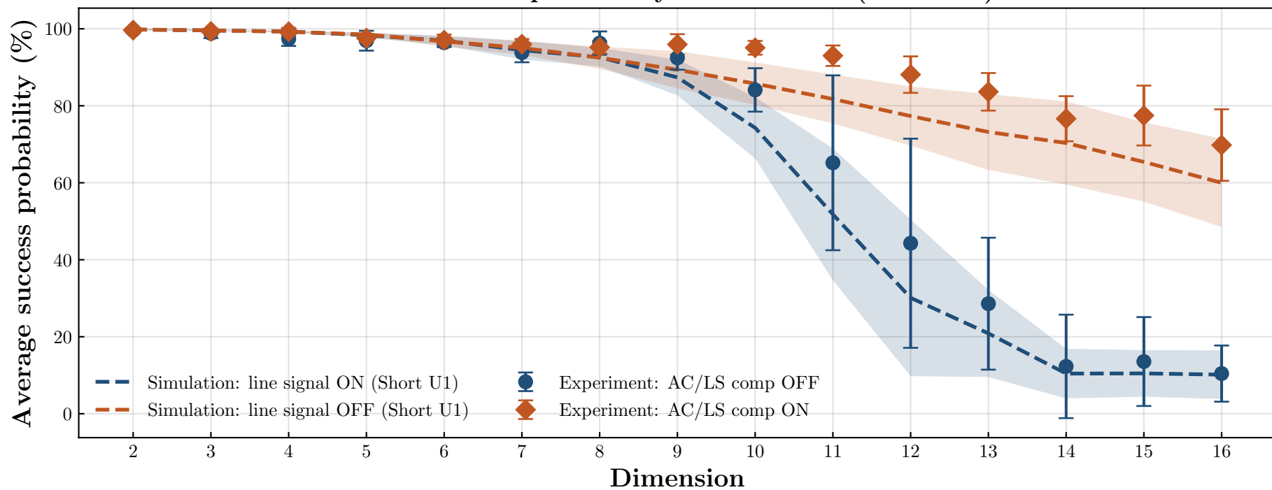
BVA success probability vs dimension (Short U1)
