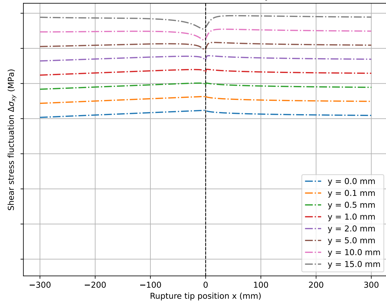
Shear stress fluctuation (xy)
