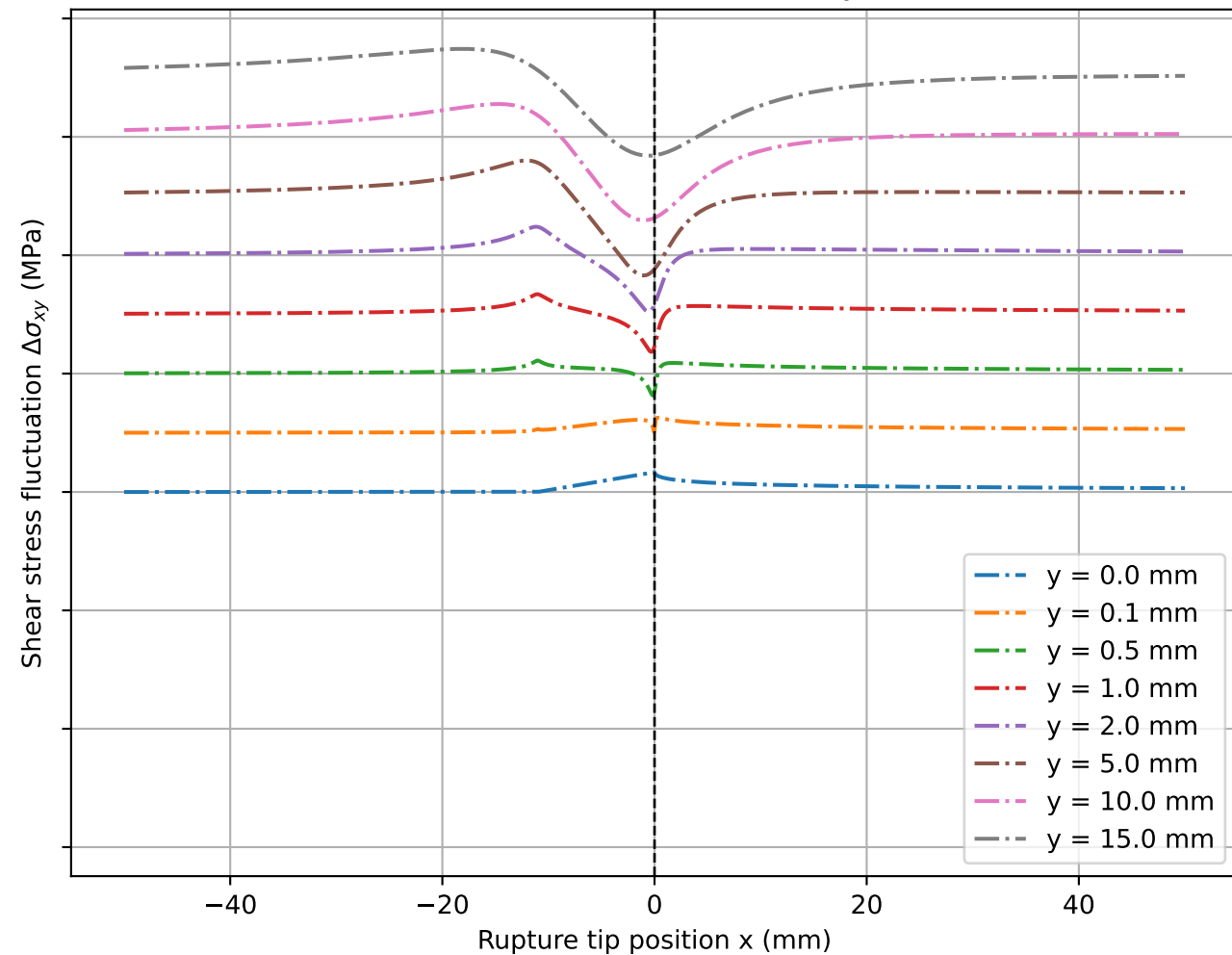
Shear stress fluctuation ( \sigma_{xy} )
