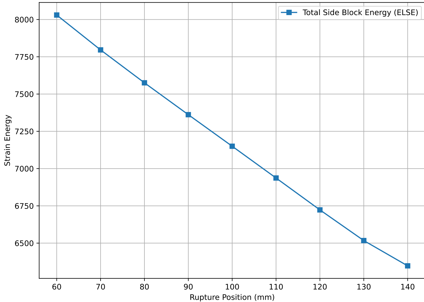
Strain Energy vs. Rupture Position
