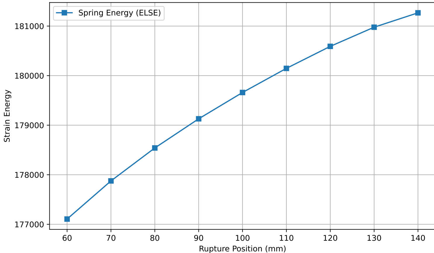
Strain Energy vs. Rupture Position
