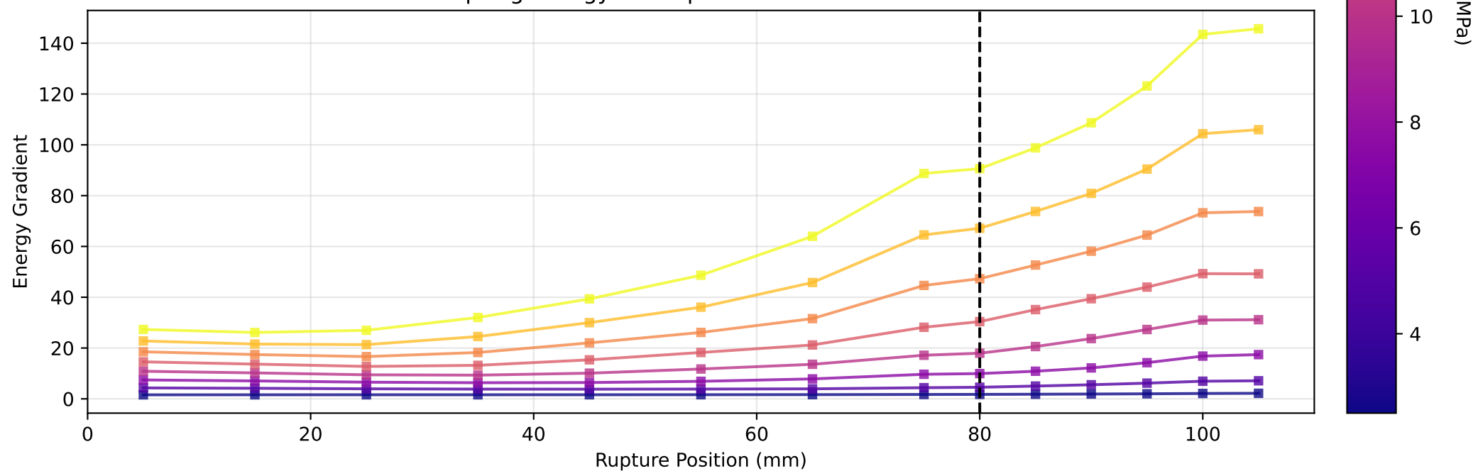
Gradient of Spring Energy vs. Rupture Position - All Normal Stresses
