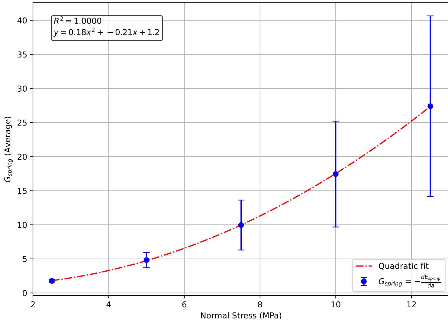
Quadratic Fit of Average Spring Energy Gradient vs. Normal Stress, Displacement Control
