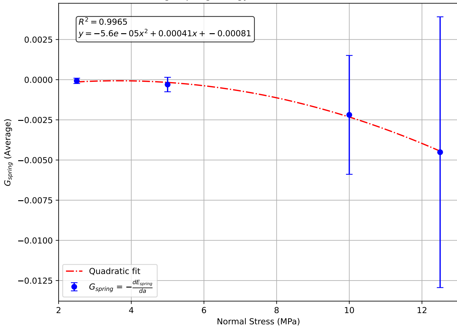
Quadratic Fit of Average Spring Energy Gradient vs. Normal Stress, Stress Control
