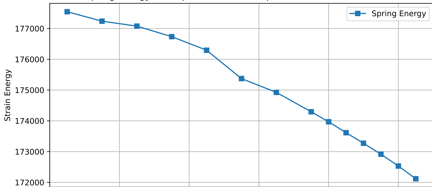
Spring Energy vs. Rupture Position, Displacement Control, 38.0MPa
